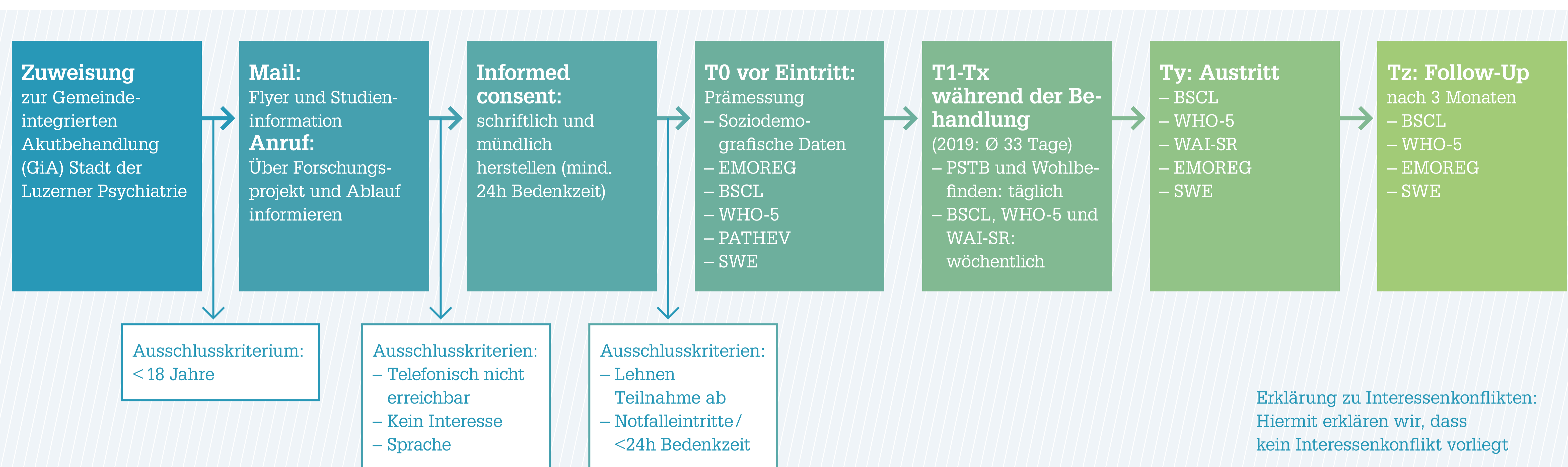
Abb. 1: Flowchart
